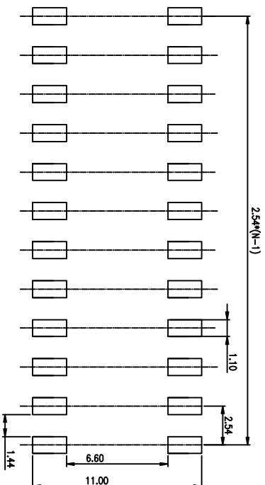
RECOMMENDED PCB LAYOUT (TOP VIEW)
